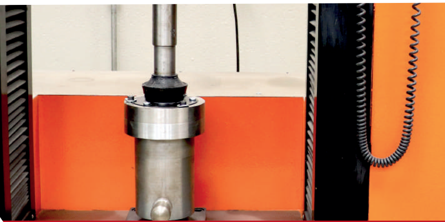
Cyclic tests
